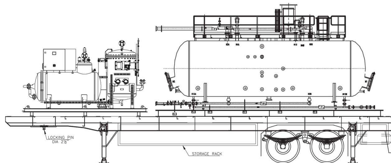
DESALTER & DEOILER
